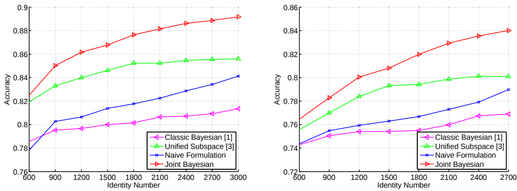
Fig. 2: Comparison with other Bayesian face related works. The joint Bayesian method is consistently better other a wide range of different training data sizes and on two databases: LFW(left) and WDFRef(right).
